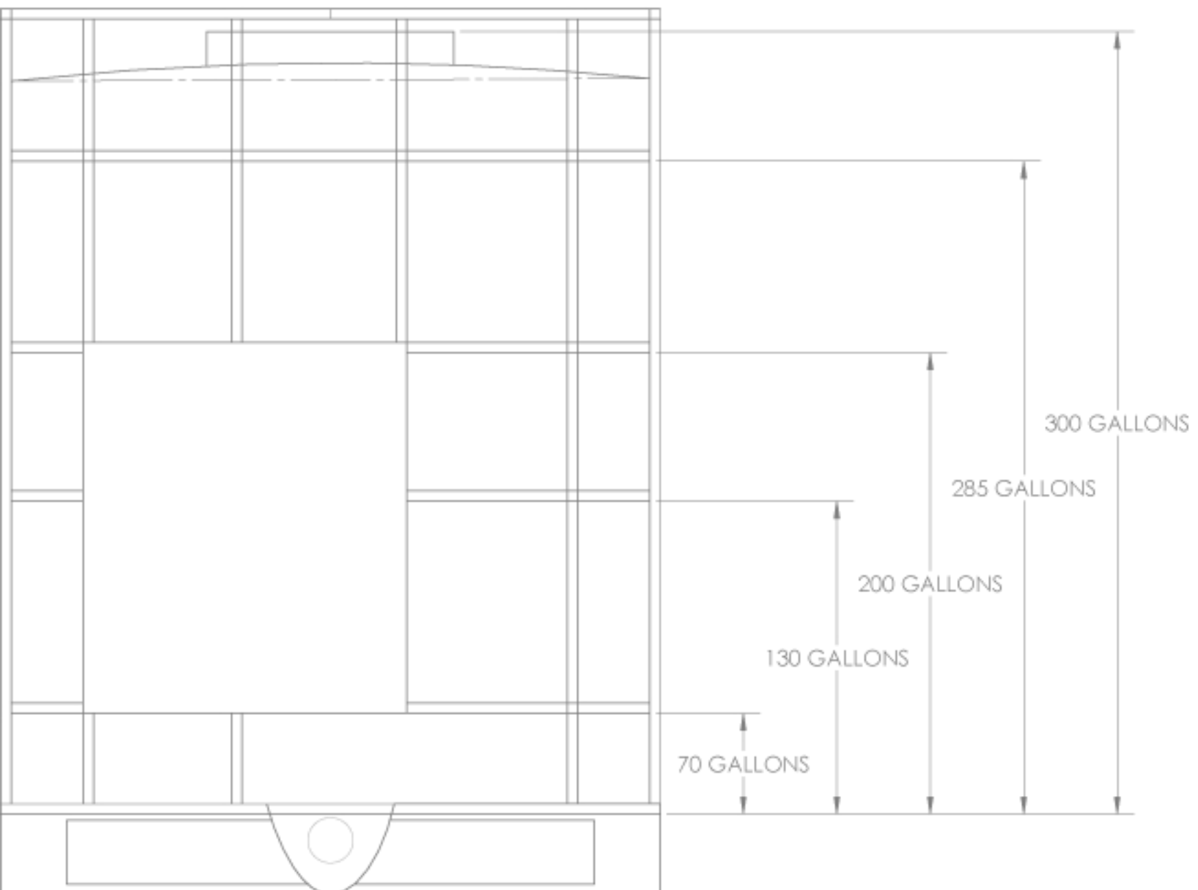
300 GALLON PALLET TANK
